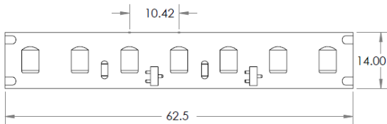
15.4w/m LED Increment 100mm LED Pitch 16.6mm
